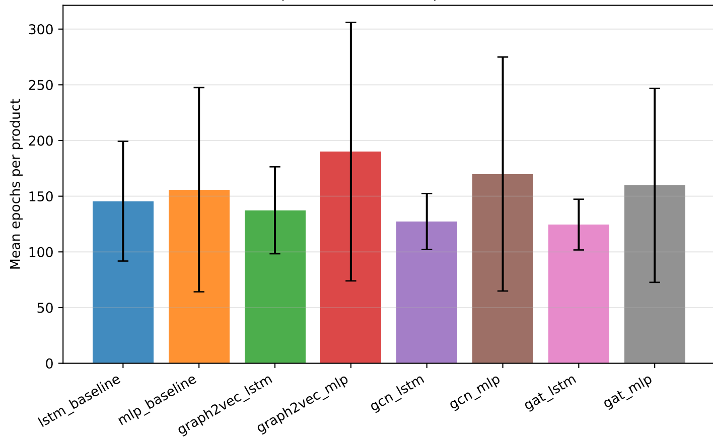
Mean epochs to train one product ( \pm std)
